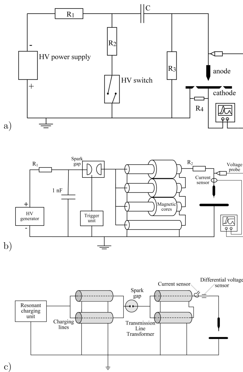
Figure 1. a) C -supply, b) TLT -supply and c) PM -supply. C -supply and TLT -supply were used in the experiments at the physics department and already described in [32]; a detailed drawing of the discharge chamber in these supplies including the current and voltage measurements is provided in Fig. 2 of [35]. The PM -supply was used in the experiments at the electrical engineering department and already discussed in [45]; the panel indicates the location of current and voltage measurements. Different diagnostics was used at the two locations as described in the text.
